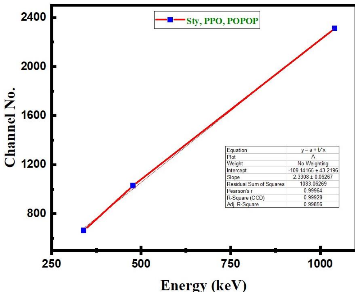
Fig. 12. Energy calibration via linear fit corresponding to the Compton edges
