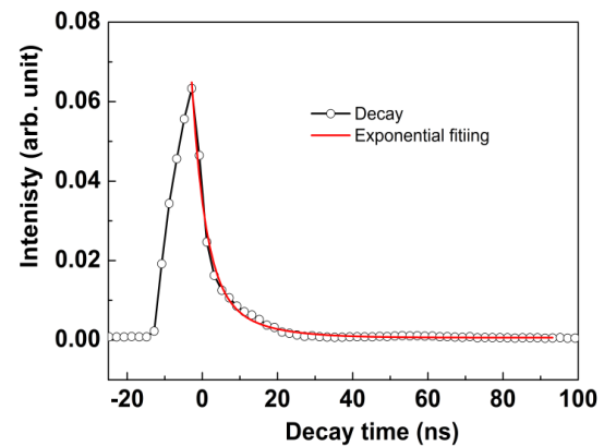
Fig. 10. Decay time curve of the polystyrene based plastic scintillator (color online)
