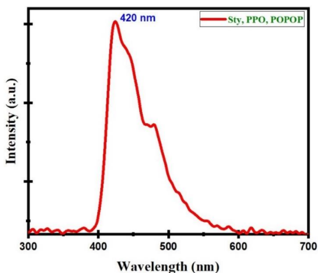
Fig. 6. Emission wavelength of the plastic scintillator (color online)
