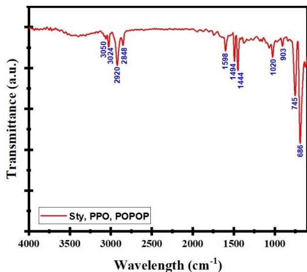
Fig. 5. FTIR spectrum of the fabricated scintillator (color online)
