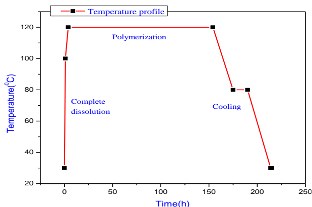
Fig. 2. Temperature profile of the synthesis process (color online)
