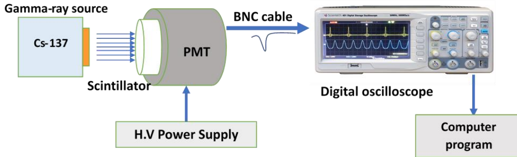
Fig. 9. The experimental setup for measuring the decay time of the plastic scintillator (color online)
