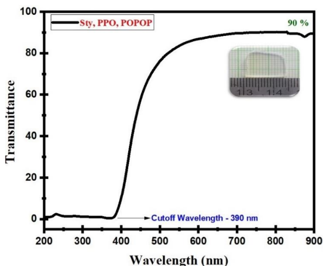
Fig. 4. Transmittance of the synthesized plastic scintillator (color online)
