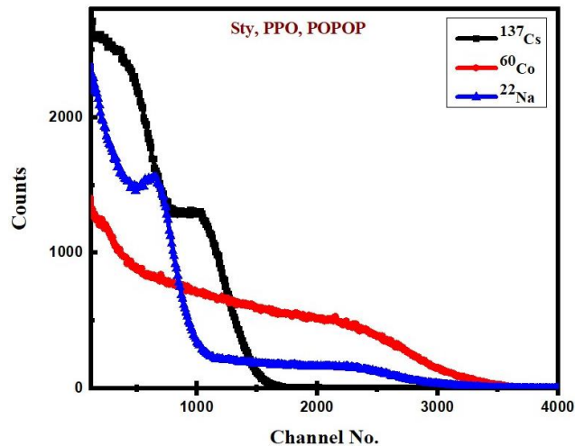
Fig. 11. Pulse height spectra using ^{137}\text{Cs} , ^{60}\text{Co} and ^{22}\text{Na} sources (color online)
