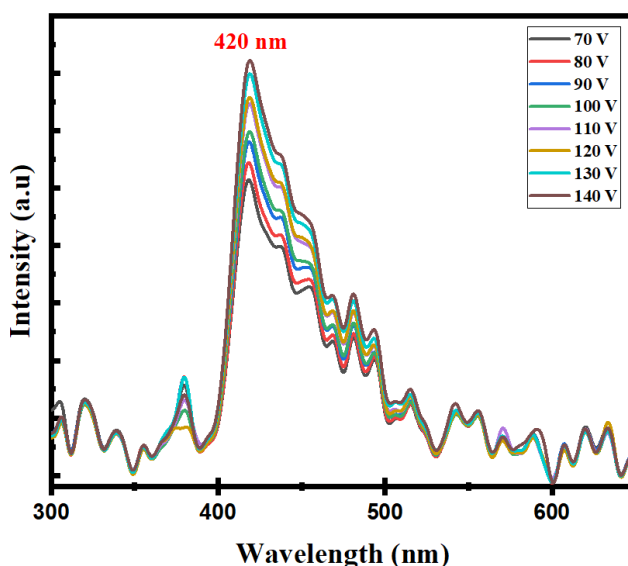
Fig. 7. Radioluminescence spectra for different voltages (color online)
